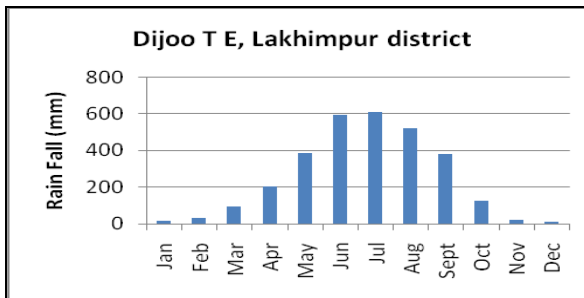
Fig.1.4: Annual variation of rainfall as recorded in six rain gauge stations of Lakhimpur district
